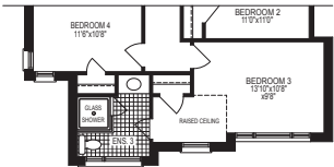
PART. OPT. 5 BEDROOM SECOND FLOOR PLAN, EL. 'B'
