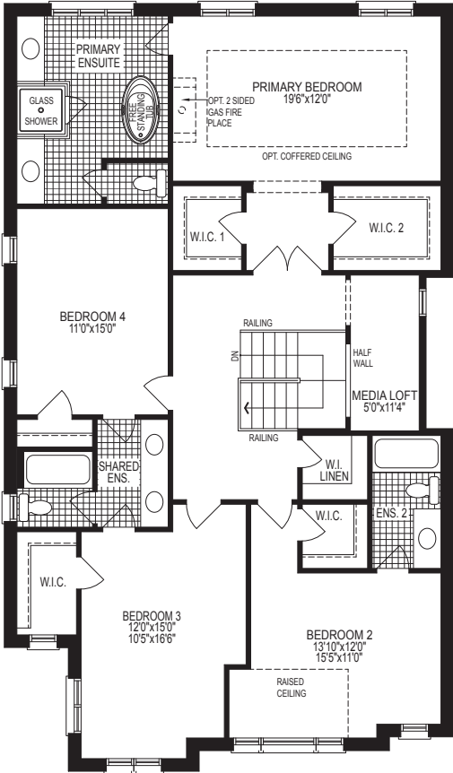
SECOND FLOOR PLAN, EL. 'A'
